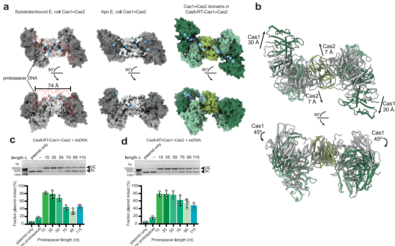
Fig. 3 Cas6-RT-Cas1–Cas2 shows length selectivity for dsDNA and ssDNA substrates for integration. a Comparison of Cas1–Cas2 disposition within the Cas6-RT-Cas1–Cas2 complex (color-coding from Fig. 1) to substrate-bound E. coli Cas1–Cas2 integrase (PDB:5D55) and apo E. coli Cas1–Cas2 integrase (PDB:4P6I) (Cas1a, dark gray; Cas1b, medium gray; Cas2, light gray), shown in surface representation. Two views are shown related by a 90° rotation. Arginine clamp and arginine channel residues are colored in blue. Protospacer substrate is depicted in red outline. b Overlay of Cas1–Cas2 domains of Cas6-RT-Cas1–Cas2 complex (color-coding from Fig. 1) with apo E. coli Cas1–Cas2 integrase (PDB:4P6I) (gray), aligned via Cas2 dimer, shown in ribbon representation. Two views are shown related by a 90° rotation. Arrows indicate conformational difference between Cas1–Cas2 domain of Cas6-RT-Cas1–Cas2 complex and that of E. coli Cas1–Cas2. c Cas6-RT-Cas1–Cas2 integration assays with variable length dsDNA protospacers (15–115 bp). Supercoiled pCRISPR plasmid that functions as target for integration (SC) and open circular products (OC) are indicated. Fraction plasmid nicked is calculated as the fraction of open circular products relative to all plasmid (error bars, mean \pm sd, n = 3 biologically independent experiments). d Cas6-RT-Cas1–Cas2 integration with variable length ssDNA protospacers (15–115 nt), quantifying fraction plasmid nicked (error bars, mean \pm sd, n = 3 biologically independent experiments). Uncropped gels and source data for panels c and d are provided as a Source Data file.
