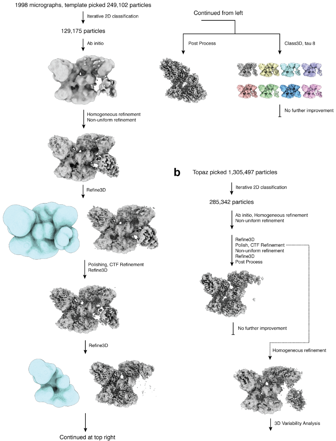
Supplementary Figure 2. Cryo-EM processing pipeline. a,b Cryo-EM data processing pipeline in RELION and cryoSPARC from RELION picked particles and Topaz picked particles respectively. Cryo-EM maps are colored gray, and masks used in RELION colored light blue. See Methods for details.
