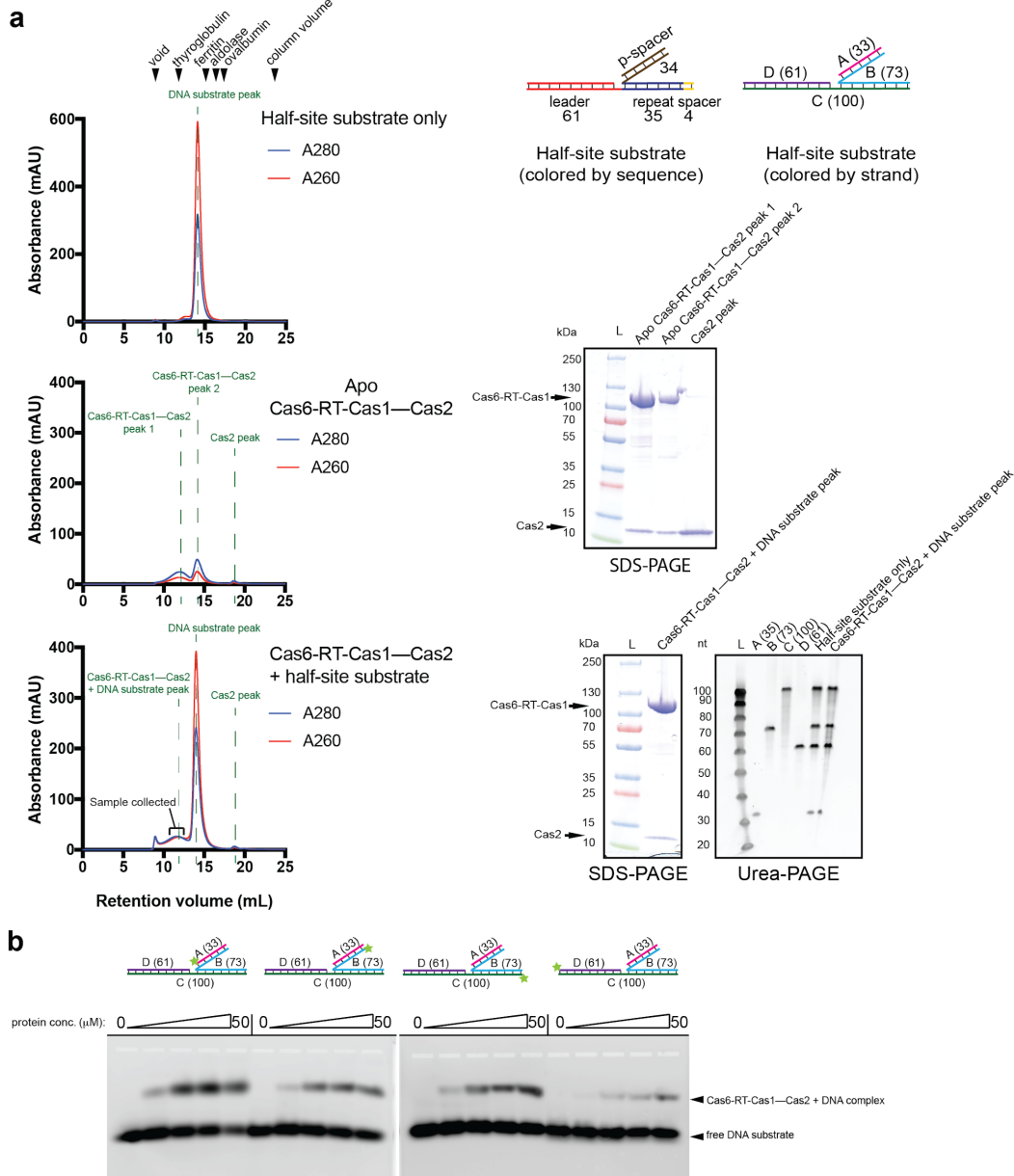
Supplementary Figure 1. Complex formation. a Gel filtration runs of DNA half-site substrate only, apo Cas6-RT-Cas1—Cas2, and Cas6-RT-Cas1—Cas2 + DNA half-site substrate. Cartoons of half-site substrate are shown colored by sequence (leader, red; repeat, blue; spacer, yellow; dsDNA protospacer, brown) and colored by strand with lengths of DNA strands shown (A, pink; B, light blue; C, green; D, purple). The absorbance at 280 nm (blue) and 260 nm (red) are shown and the void volume, column volume, and elution volumes of standard proteins are indicated by black arrowheads. The peaks representing the Cas6-RT-Cas1—Cas2 complexes, the sample used for cryo-EM data collection, and free DNA substrate are indicated by green dashed lines. SDS-PAGE gels and urea-PAGE gel of the elution samples are provided. Source data are provided as a Source Data file. b Electrophoretic mobility shift assays using fluorescent half-site substrates colored by strand with color-coding from a . Star indicates 6-carboxyfluorescein label. Results are representative of 3 independent experiments. Uncropped gels are available in a Source Data file.
