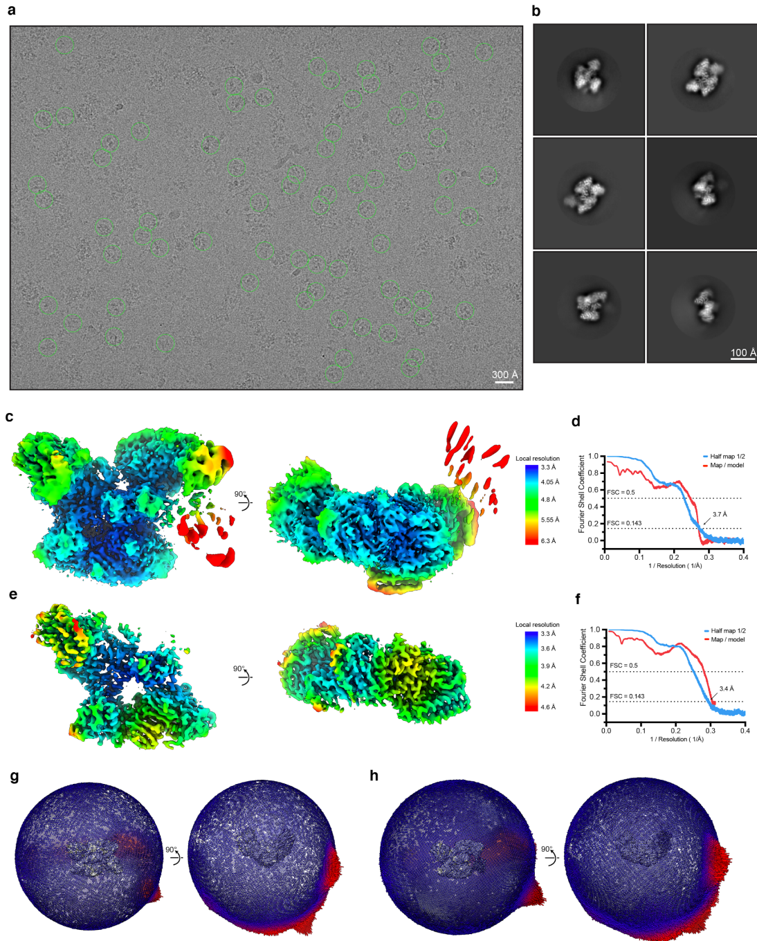
Supplementary Figure 3. Cryo-EM validation. a Representative micrograph with 10 Å lowpass filter, particles which contributed to the final reconstruction are circled. b Selected 2D class averages. Results for a and b are representative of 1996 micrographs (Supplementary Table 3). All micrographs are deposited in EMPIAR-10642 [ https://dx.doi.org/10.6019/EMPIAR-10642 ]. c, e Local resolution estimated in RELION3.1 with map surfaces colored in rainbow as indicated, for full and partial complexes respectively. d, f Fourier Shell Correlation (FSC) for the two unfiltered half-maps (light blue) and final map versus model (red), for full and partial complexes respectively. Source data are provided as a Source Data file. g, h Angular distribution of particles with corresponding cryo-EM map, for full and partial complexes respectively.
