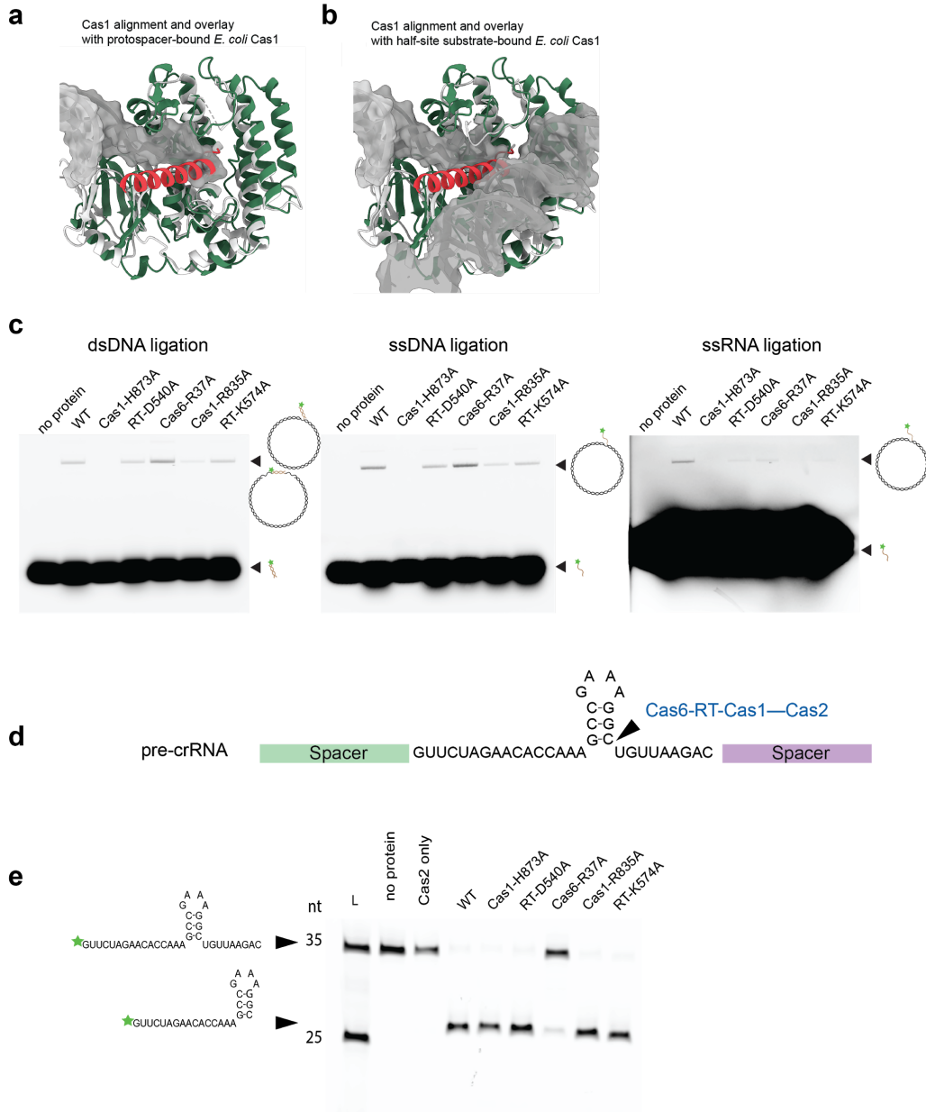
Supplementary Figure 8. Crosstalk between Cas1, RT, and Cas6 domains. a Alignment and overlay of Cas1a domain (dark green) with Cas1a from protospacer-bound E. coli Cas1—Cas2 structure (white, PDB: 5DS5 [ https://doi.org/10.2210/pdb5ds5/pdb ]). Protospacer substrate shown in gray surface representation. RT-helix is colored red. b Alignment and overlay of Cas1a domain (dark green) with Cas1a from half-site substrate-bound E. coli Cas1—Cas2 structure (white, PDB: 5VVJ [ https://doi.org/10.2210/pdb5vvj/pdb ]). Half-site substrate shown in gray surface representation. c Ligation of fluorescent 35-nt dsDNA (0.5 \mu M), ssDNA (0.5 \mu M), and ssRNA (4 \mu M) protospacer into target pCRISPR by WT and mutant Cas6-RT-Cas1—Cas2s. Integration products and free protospacer are indicated and schematized. Star indicates 6-carboxyfluorescein label. d Sequence and predicted secondary structure of repeat with predicted cleavage site indicated. e crRNA processing activity assay comparing WT and mutant Cas6-RT-Cas1—Cas2s. Sequence and predicted secondary structure of CRISPR repeat RNA and the predicted product are indicated. Star indicates 6-carboxyfluorescein label. Results for c and e are representative of 3 independent experiments. Uncropped gels are available in a Source Data file.
