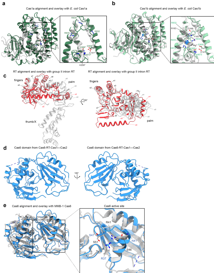
Supplementary Figure 4. Architecture of Cas1, RT, and Cas6 domains. a Alignment and overlay of Cas1a domain (dark green) from Cas6-RT-Cas1—Cas2 structure with E. coli Cas1a (white, PDB: 5DS5 [ https://doi.org/10.2210/pdb5ds5/pdb ]) and closeup of active site and surrounding residues, shown in stick configuration. Cas6-RT-Cas1—Cas2 residues are labeled in dark green, E. coli Cas1 residues labeled in black. Active site residues are labeled with an asterisk *. b Alignment and overlay of Cas1b domain (turquoise) with E. coli Cas1b (white, PDB: 5DS5 [ https://doi.org/10.2210/pdb5ds5/pdb ]) and closeup of active site and surrounding residues. c Alignment and overlay of RT domain (red) and group II intron RT (white, PDB: 6AR1 [ https://doi.org/10.2210/pdb6AR1/pdb ]) with helices from the finger and palm domains labeled. Closely-aligned helices labeled in black, offset helices labeled in red (Cas6-RT-Cas1—Cas2 RT domain) and gray (group II intron RT). d Architecture of Cas6 domain from Cas6-RT-Cas1—Cas2 structure and 90° rotation. e Alignment and overlay of Cas6 domain from Cas6-RT-Cas1—Cas2 structure (blue) with Cas6 domain from MMB-1 Cas6-RT-Cas1 fusion (PDB: 6DD5 [ https://doi.org/10.2210/pdb6DD5/pdb ], white) and closeup of active site residues, shown in stick configuration. Cas6-RT-Cas1—Cas2 residues are labeled in blue, MMB-1 Cas6 residues labeled in black.
