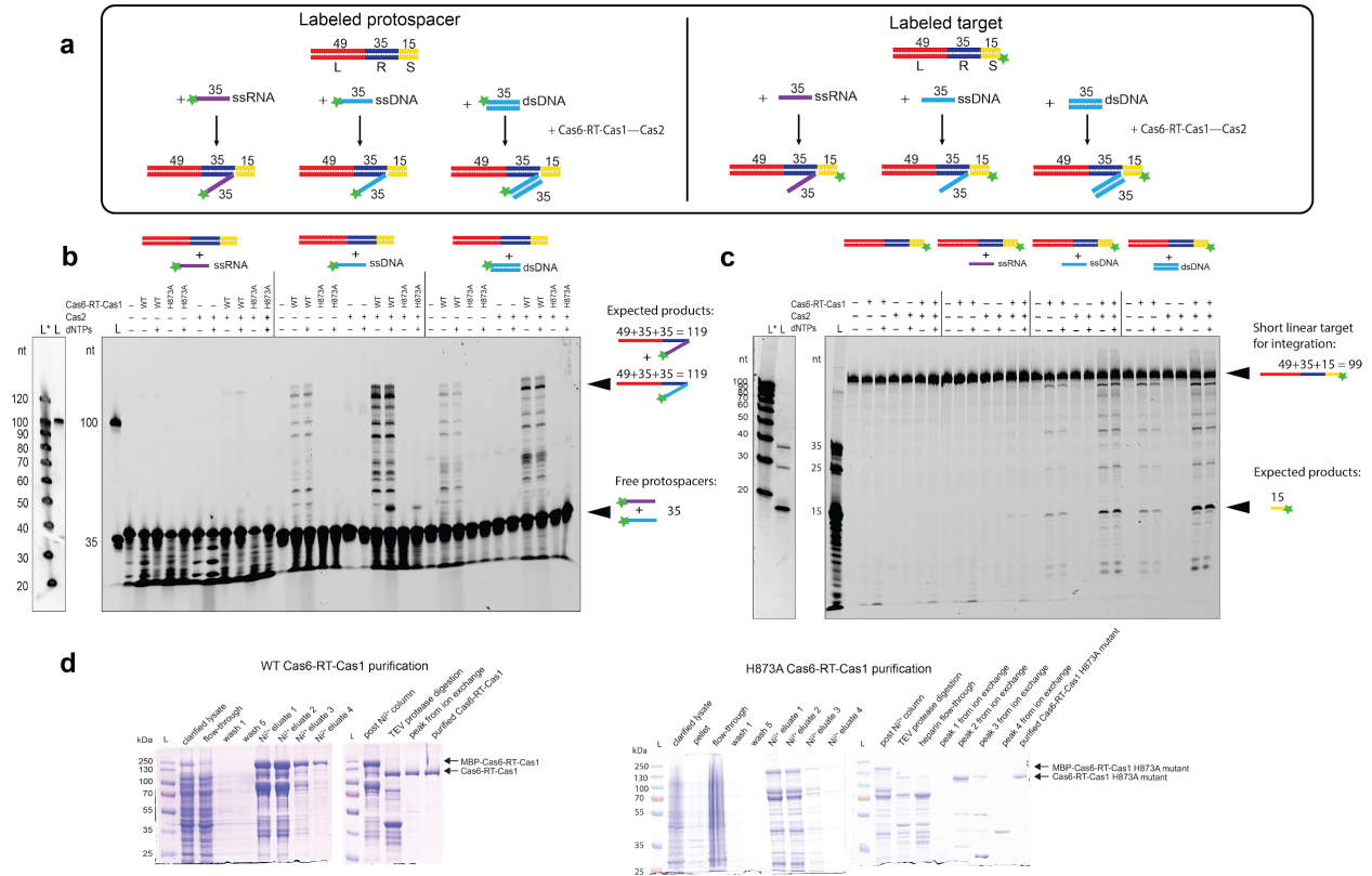
Supplementary Figure 6. Cas6-RT-Cas1—Cas2 catalyzes ligation of DNA and RNA protospacers into the CRISPR array. a Schematic of in vitro integration reaction of DNA or RNA protospacer into a short linear dsDNA containing the CRISPR repeat as the target for integration. The lengths of the leader (L, red), repeat (R, dark blue), spacer (S, yellow), and protospacers (DNA, light blue; RNA, purple) are indicated. Star indicates 6-carboxyfluorescein label. b Cleavage-ligation assays conducted with fluorescent dsDNA, ssDNA, and ssRNA protospacers (1 \mu M) and unlabeled short linear target containing the CRISPR repeat. Expected products and their lengths are indicated. On the left, a non-fluorescent ladder L* is shown next to the fluorescent ladder L, visualized after SYBR Gold poststaining. c Cleavage-ligation assays conducted with fluorescent target (bottom strand labeled). Expected products and their lengths are indicated. Results for b and c are representative of 3 independent experiments. d SDS-PAGE gels of WT Cas6-RT-Cas1 and H873A Cas6-RT-Cas1 mutant purifications, representative of 1 independent experiment. Uncropped gels are available in a Source Data File.
